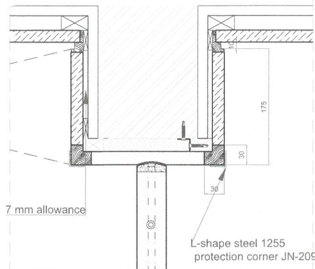
D5 Junction details
