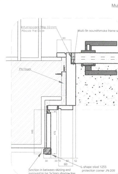
D3 Typical Frame detail
